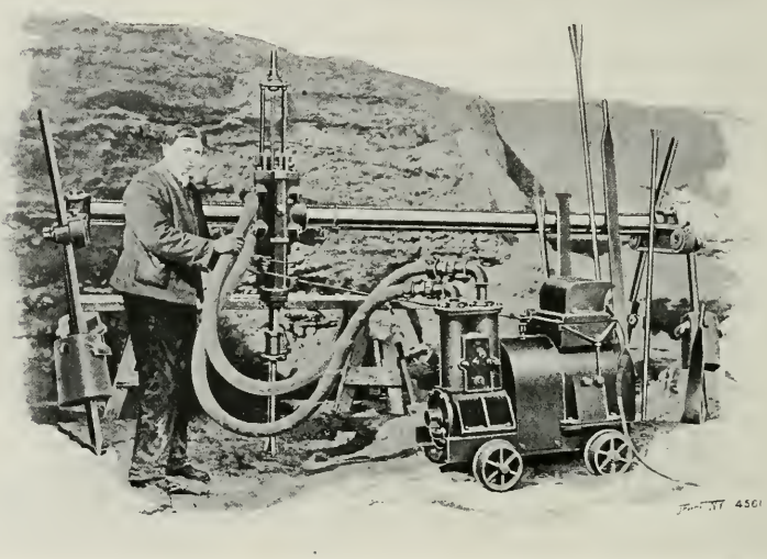
"Electric-Air" Rock Drill on Quarry Bar Mounting.
